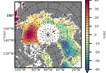
Mean DOT from Armitage et al. 2013
