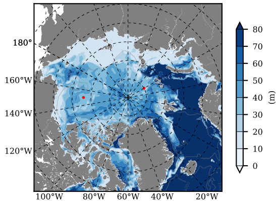
BCTTWINERA5SS mean MLD01 over 2001 m03
