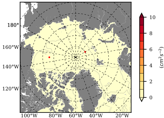
BCTTWINERA5SSDGTK mean EKE @ 0 m over 1995
