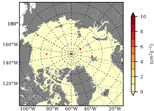
BCTTWINERA5SSDGTK mean EKE @ 0 m over 1998
