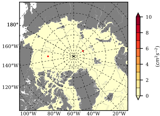
BCTTWINERA5SSNVC mean EKE @ 0 m over 1997
