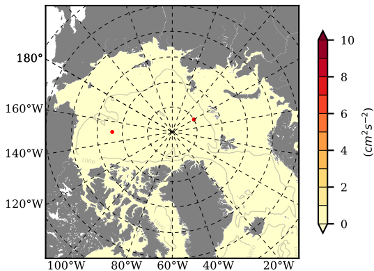
BCTTWINERA5SSNVC mean EKE @ 0 m over 2002
