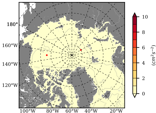
BCTTWINERA5SSNVC mean EKE @ 0 m over 2004
