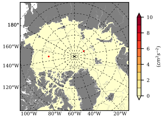
BCTTWINERA5SSNVC mean EKE @ 0 m over 2011
