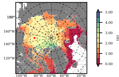
NSIDC mean SICON m03 1999
