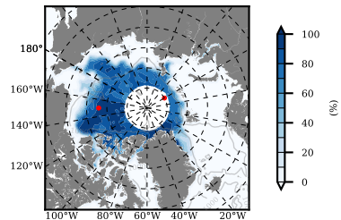
NSIDC mean SICON m09 1999
