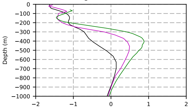
2012 mean temperature @ moor Arctic B box
