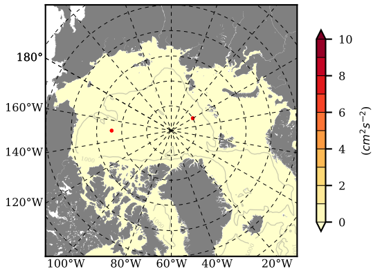
BCTTWINERA5SSRW mean EKE @ 0 m over 2006
