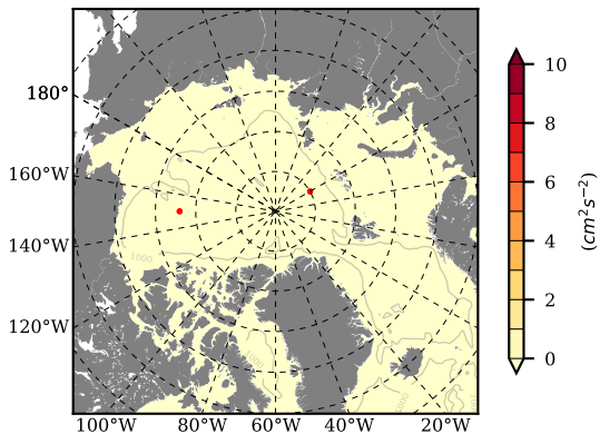
BCTTWINERA5SSRW mean EKE @ 0 m over 2011
