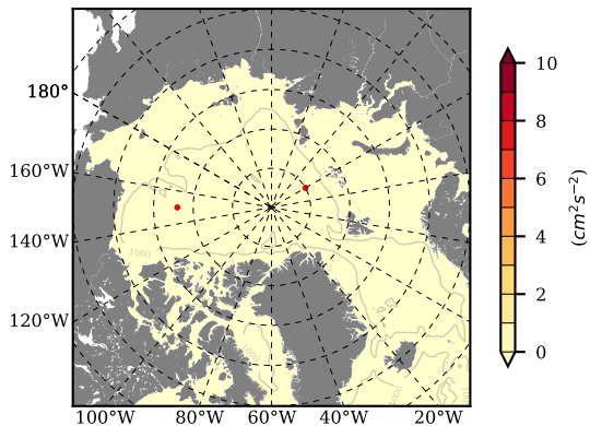
BCTTWINERA5SSRW mean EKE @ 0 m over 2016
