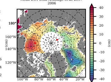
Mean DOT from Armitage et al. 2017 2006
