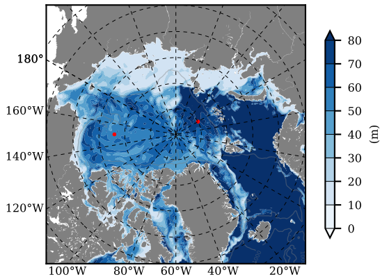
BCTTWINERA5SSRW mean MLD01 over 2013 m03
