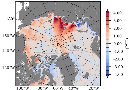
BCTTWINERA5SSRW mean Sal diff with init. state over 1995 @ depth 0 m
