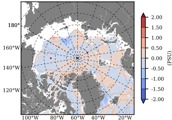
BCTTWINERA5SSRW mean Sal diff with init. state over 1995 @ depth 97 m
