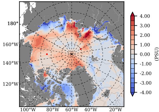
BCTTWINERA5SSRW mean Sal diff with init. state over 2000 @ depth 0 m
