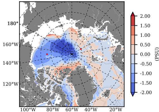
BCTTWINERA5SSRW mean Sal diff with init. state over 2005 @ depth 97 m
