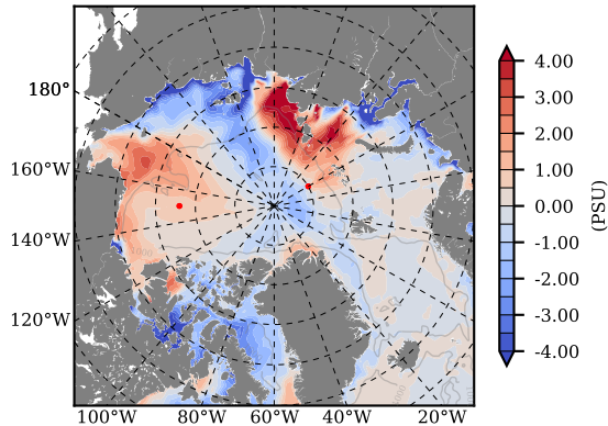
BCTTWINERA5SSRW mean Sal diff with init. state over 2005 @ depth 0 m
