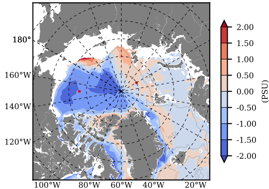
BCTTWINERA5SSRW mean Sal diff with init. state over 2010 @ depth 97 m
