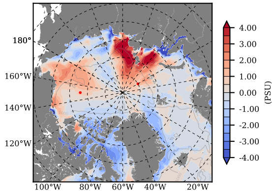
BCTTWINERA5SSRW mean Sal diff with init. state over 2012 @ depth 0 m
