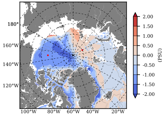
BCTTWINERA5SSRW mean Sal diff with init. state over 2014 @ depth 97 m
