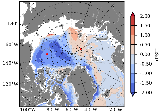
BCTTWINERA5SSRW mean Sal diff with init. state over 2015 @ depth 97 m
