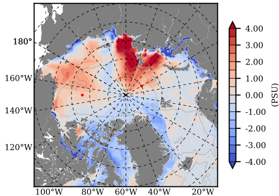
BCTTWINERA5SSRW mean Sal diff with init. state over 2016 @ depth 0 m
