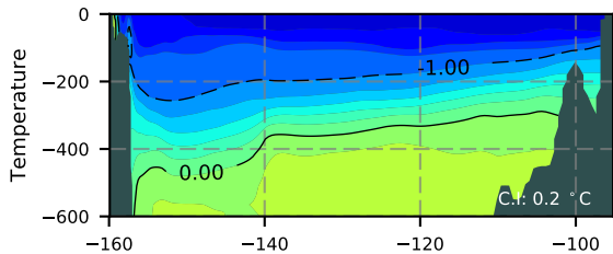
BCTTWINERA5SSRW / Beaufort Section 2016
