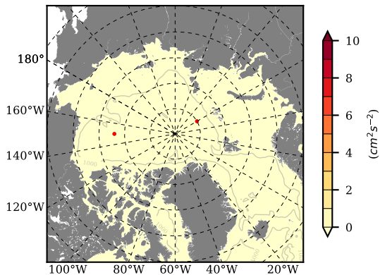
BCTTWINERA5SSTKE mean EKE @ 0 m over 1995
