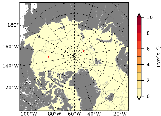
BCTTWINERA5SSTKE mean EKE @ 0 m over 1997
