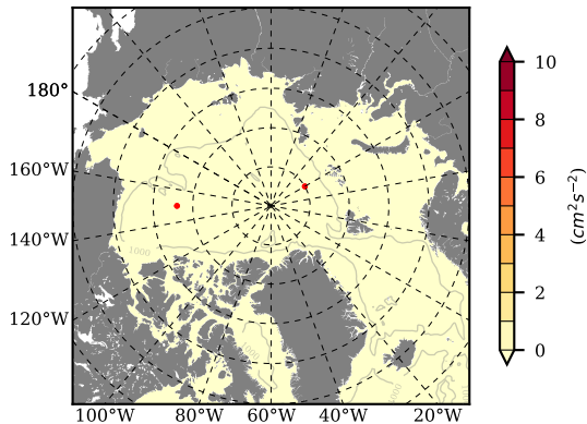
BCTTWINERA5SSTKE mean EKE @ 0 m over 1998
