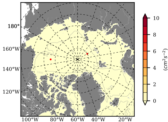
BCTTWINERA5SSTKE mean EKE @ 0 m over 1999
