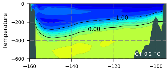
BCTTWINERA5SSTKE / Beaufort Section 1999
