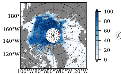
NSIDC mean SICON m09 1995
