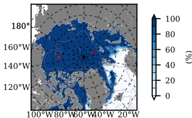
mean SICON m03
