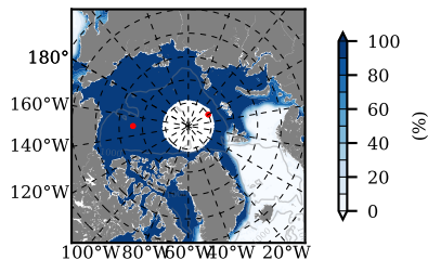
NSIDC mean SICON m09 1998
