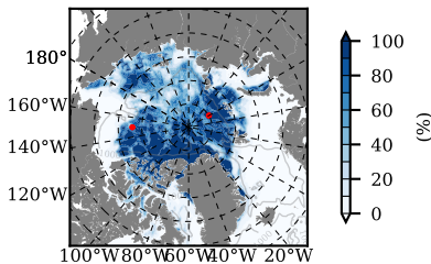
mean SICON m09
