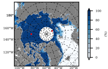
NSIDC mean SICON m09 2013
