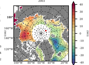
Mean DOT from Armitage et al. 2017 2003
