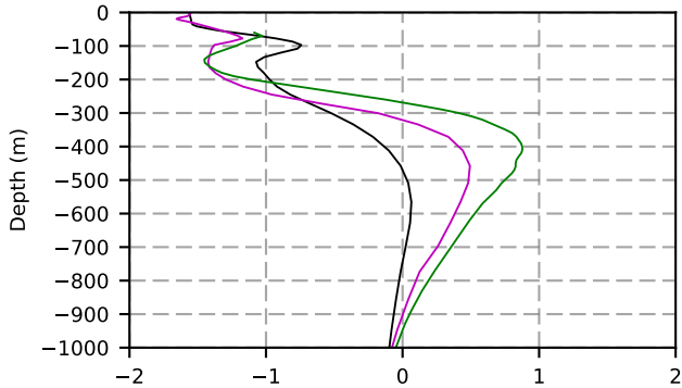
2016 mean temperature @ moor Arctic B box
