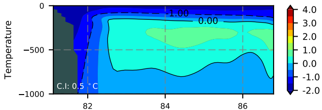
ILBOXE68 / Kara Section 2002
