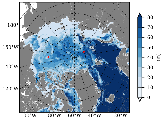
ILBOXE69 mean MLD01 over 2014 m03
