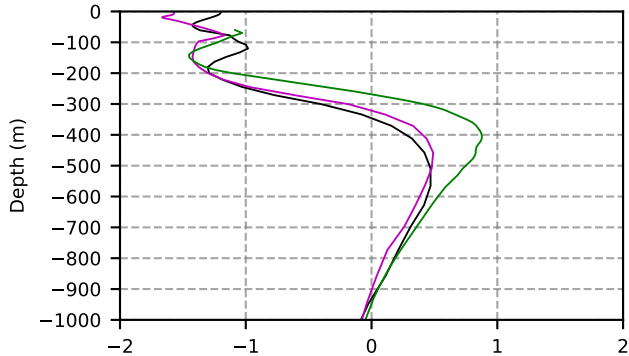
2049 mean temperature @ moor Arctic B box
