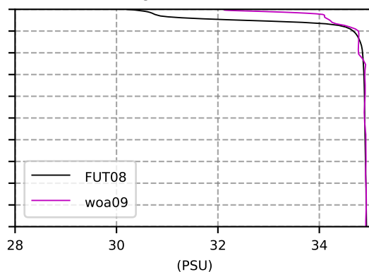
@ moor EUR box
