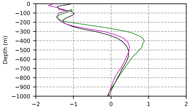
2050 mean temperature @ moor Arctic B box
