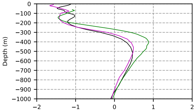
2053 mean temperature @ moor Arctic B box
