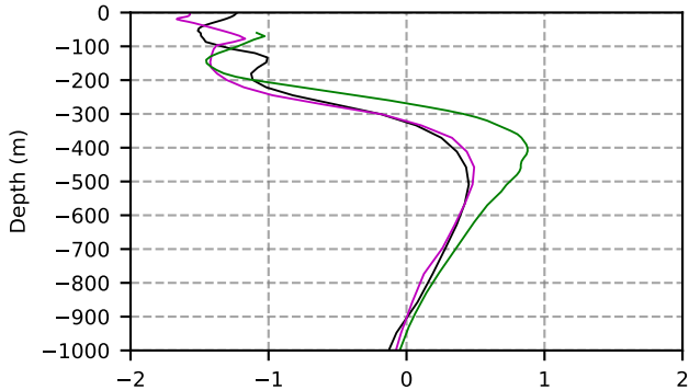
2056 mean temperature @ moor Arctic B box
