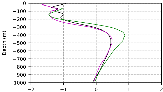
2061 mean temperature @ moor Arctic B box
