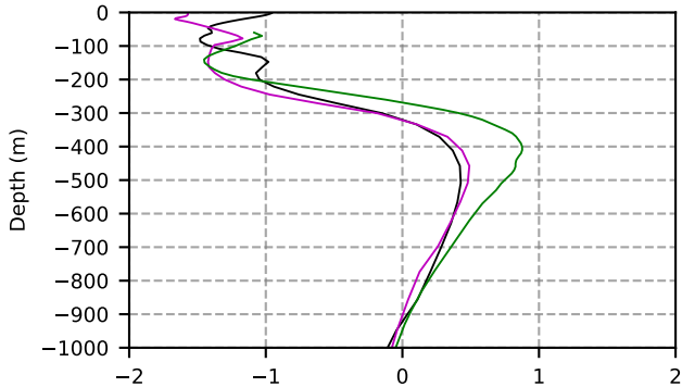
2062 mean temperature @ moor Arctic B box
