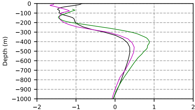
2066 mean temperature @ moor Arctic B box
