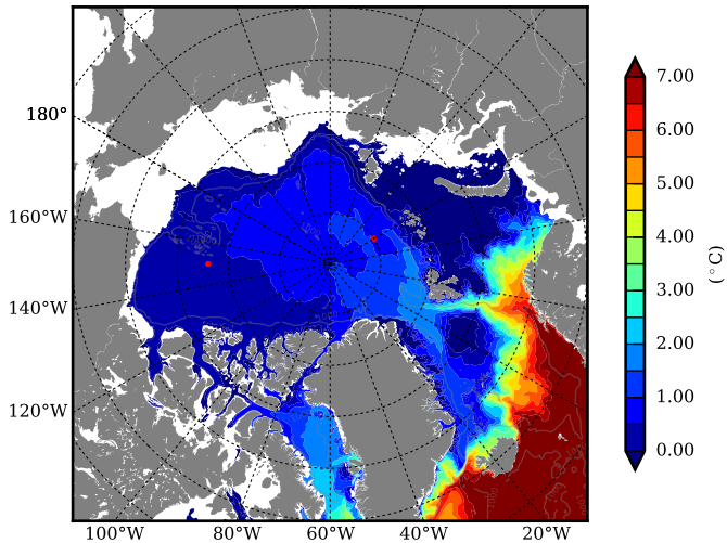
REF02 AW Max Temp over 1982
