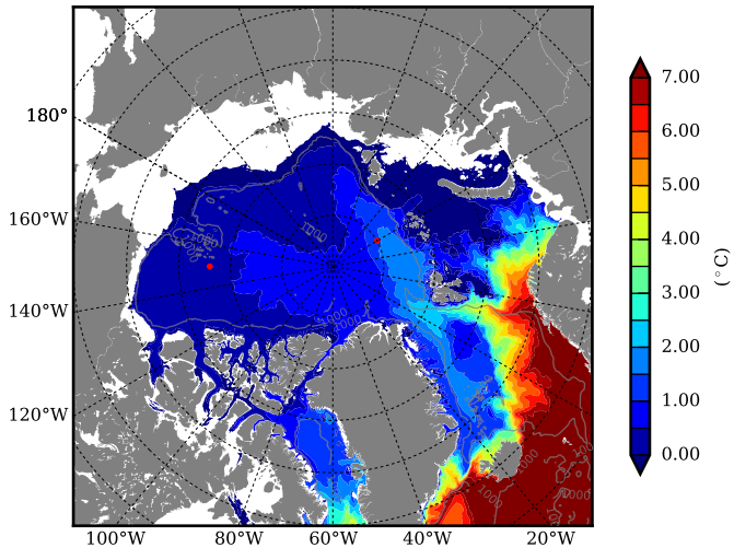
REF02 AW Max Temp over 1988
