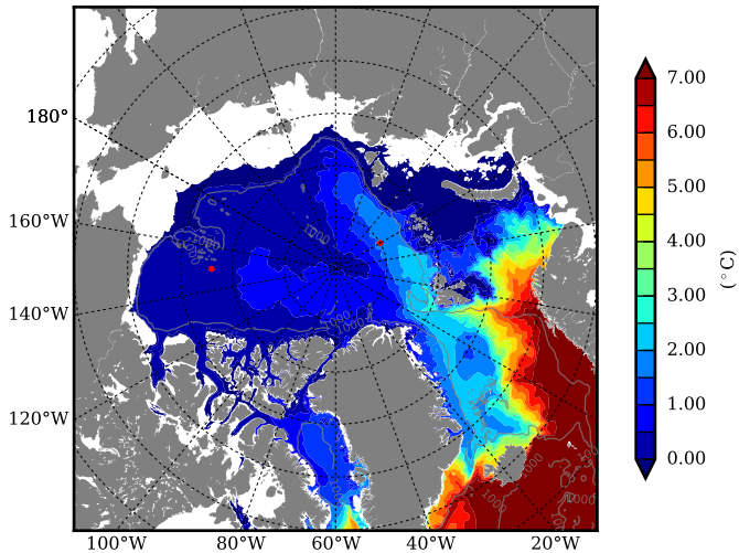
REF02 AW Max Temp over 1991
