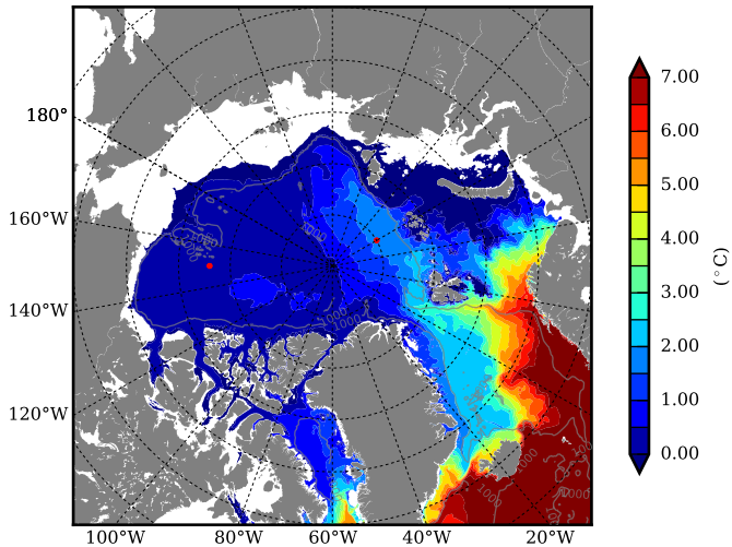
REF02 AW Max Temp over 1994
