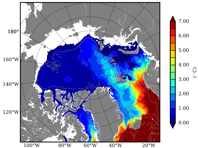
REF02 AW Max Temp over 1996
