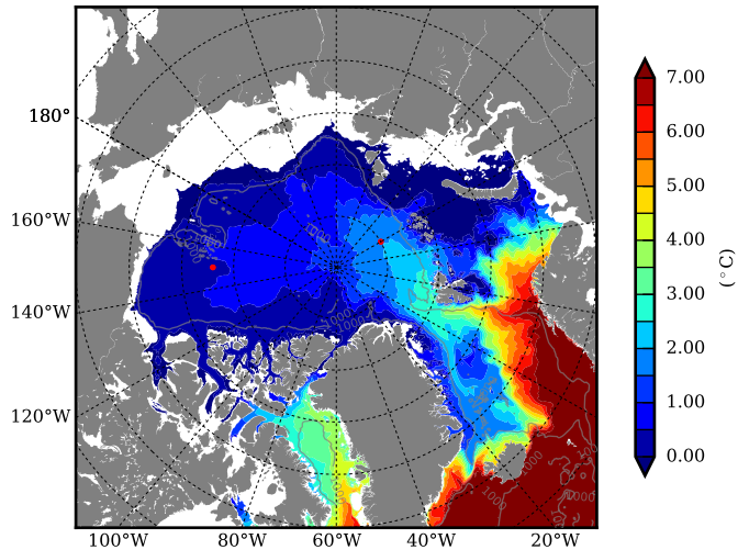
REF02 AW Max Temp over 2010
