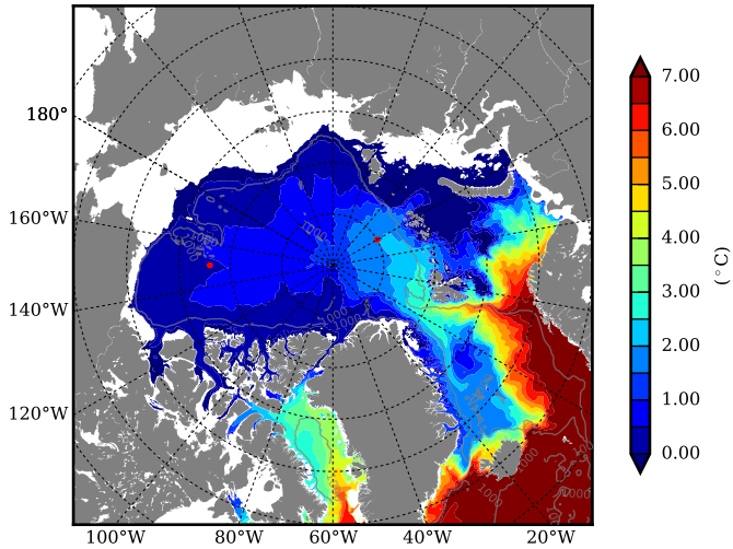
REF02 AW Max Temp over 2011
